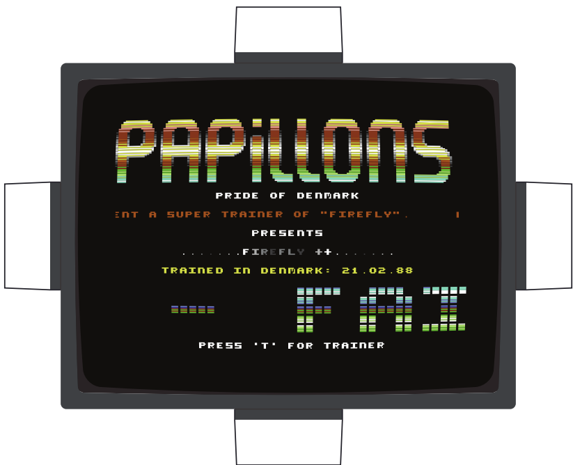
Cracktro Screens
